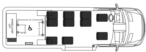
Transit Nugget - 9 Passenger 1 Wheel Chair
