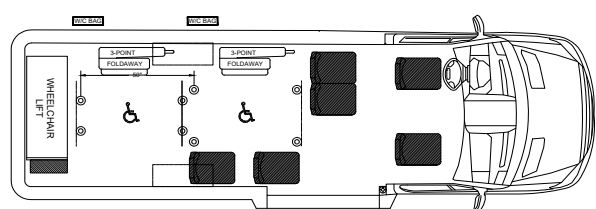
Transit Nugget - 5 Passenger 2 Wheel Chair
